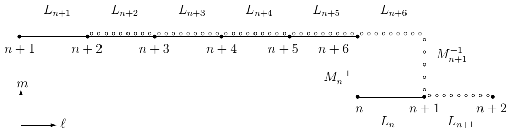
Figure 1. Standard staircase (—) and shifted staircase (ooooo) under n \rightarrow n + 1 , in the case z_1 = 1, z_2 = 6 .
